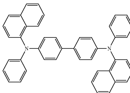
[NPB]
