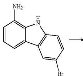
[Compound 14-B]
