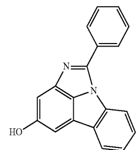
[Compound 15-D]
