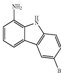
[Compound 14-B]
