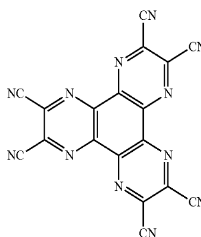
[HAT]
