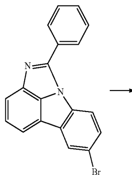
[Compound 14-C]
