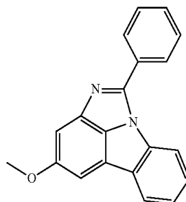
[Compound 15-C]
