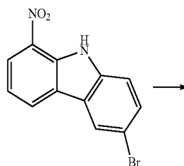
[Compound 14-A]
