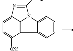
[Compound 17-E]
