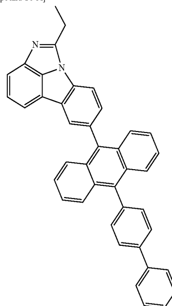
[Compound 16-A]
