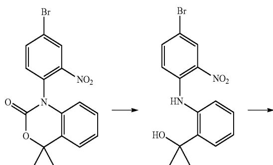
[Compound 6-A]
