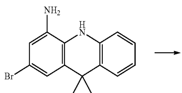
[Compound 6-D]
