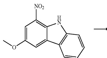
[Compound 15-A]
