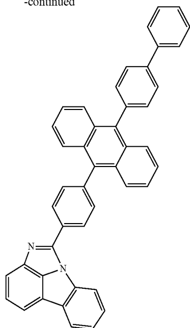
[Chemical Formula 2-5]
