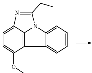
[Compound 17-C]
