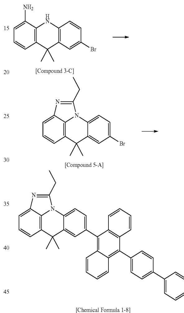
[Chemical Formula 1-8]
