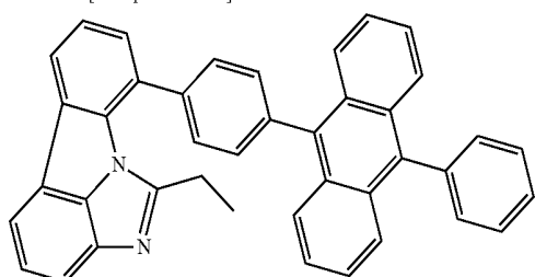
[Chemical Formula 2-22]
