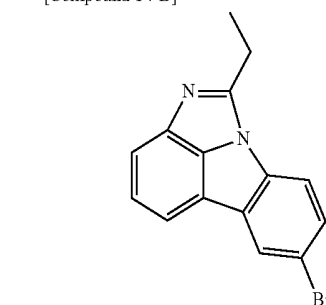
[Compound 16-A]
