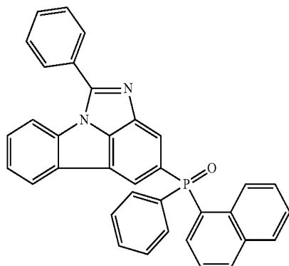
[Chemical Formula 2-25]
