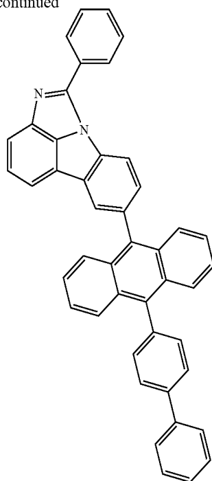
[Chemical Formula 2-6]
