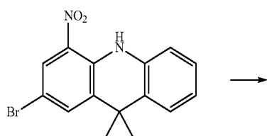
[Compound 6-C]
