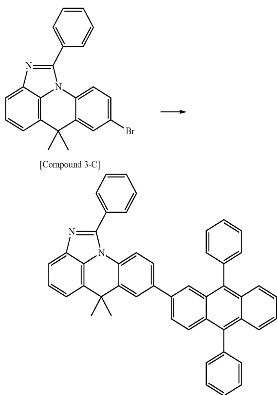
[Chemical Formula 1-11]
