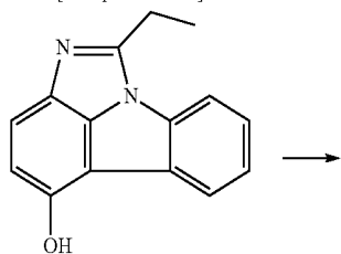
[Compound 17-D]
