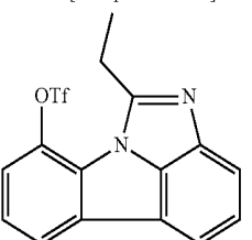
[Compound 21-E]
