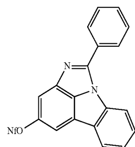
[Compound 15-E]
