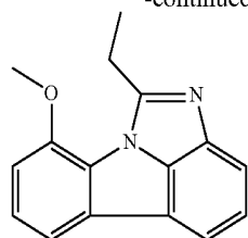
[Compound 21-C]
