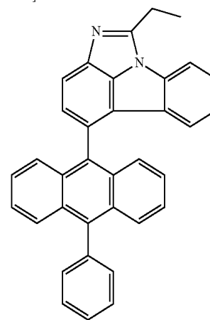
[Chemical Formula 2-15]
