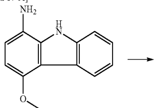
[Compound 17-B]
