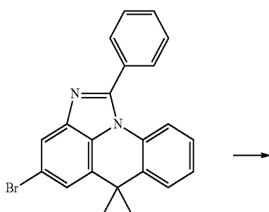
[Compound 6-E]
