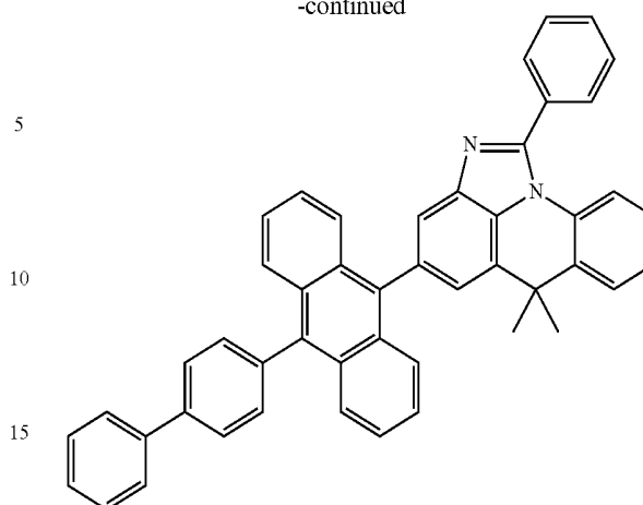
[Chemical Formula 1-4]
