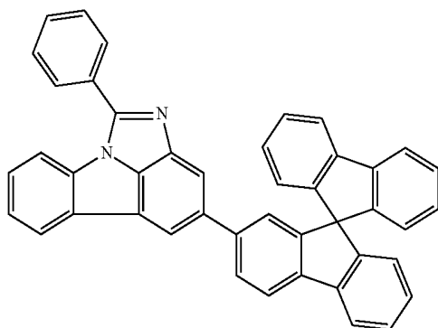
[Chemical Formula 2-25]
