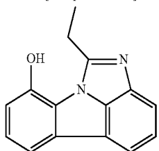
[Compound 21-D]
