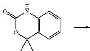
[Compound 1-B]
